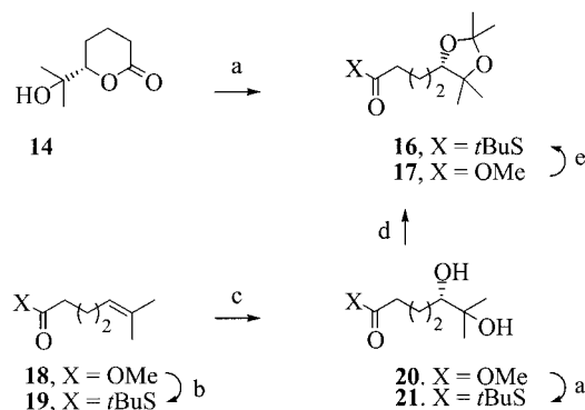
Scheme 4. The synthesis of optically active side-chain precursors; C20–C27 unit. Reagents and conditions: (a) 1. \text{AlMe}_3/t\text{BuSH} ; 2. 2,2-dimethoxypropane, \text{TsOH} , 56%, 96% ee ; (b) as reported; [36] (c) Sharpless asymmetric dihydroxylation, 18 into 20 : AD-mix- \alpha , 76% yield (after distillation), > 95% ee ; 19 into 21 : DHQ-PHAL, \text{K}_3\text{Fe}(\text{CN})_6 , \text{K}_2\text{CO}_3 , \text{OsO}_4 , 54%, 96% ee and 14 , 8%; (d) 2,2-dimethoxypropane, \text{TsOH} , 16 , 89%, 17 , 96%; (e) \text{AlMe}_3/t\text{BuSH} , 76%
