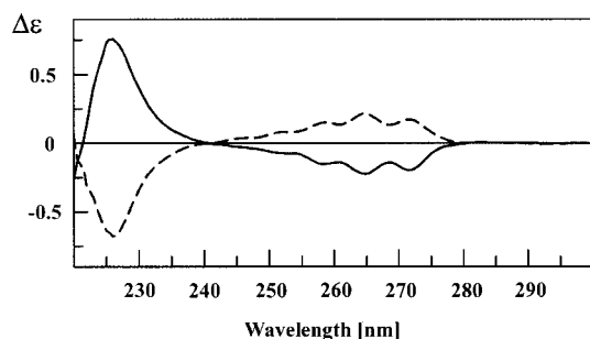
Figure 3. CD spectra of 8 (solid line) and epi-8 (dashed line)
