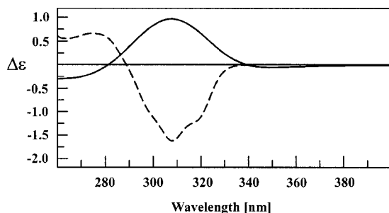
Figure 2. CD spectra of 45 (solid line) and 29 (dashed line)
