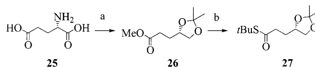
Scheme 6. The synthesis of optically active precursors of the side chain lacking gem -dimethyl groups. Reagents and conditions: (a) as reported [42,43] (b) \text{AlMe}_3/t\text{BuSH} , 47%
