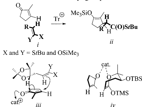
Scheme 12. Stereochemistry of the conjugate-addition reactions
