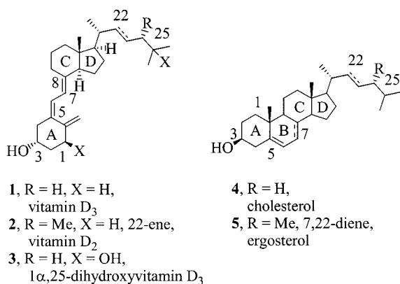
Figure 1. The most important representatives of the vitamin D group, and their respective biosynthetic and synthetic precursors
