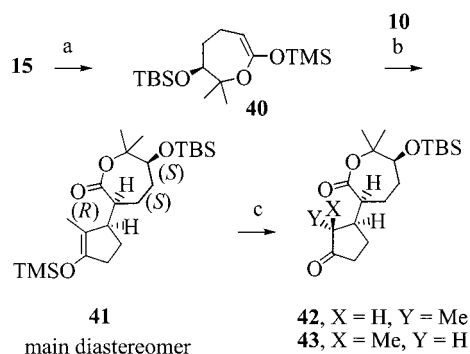
Scheme 9. Attempted use of ketene acetal 40 for the synthesis of 8 . Reagents and conditions: (a) LDA and then TMSCl, 92%; (b) TrSbCl 6 , 69%; (c) Amberlyst-15H, crystallization
