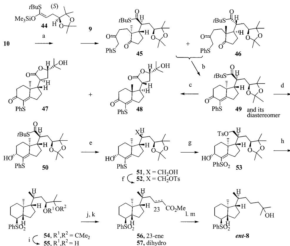
Scheme 10. Synthesis of ent -8 from ketene acetal 44 . Reagents and conditions: (a) \text{TrSbCl}_6 , 7 mol %; 75%, isomer ratio 85:11 4; (b) \text{KOH}/\text{MeOH} , 79%; (c) \text{Amberlyst-15H}/\text{MeOH} ; (d) \text{CeCl}_3 \cdot 7\text{H}_2\text{O}/\text{NaBH}_4/\text{MeOH} and crystallization, 66%; (e) \text{LiAlH}_4 ; (f) \text{TsCl}/\text{DMAP}/\text{Et}_3\text{N} ; (g) m\text{CPBA} ; (h) \text{LiAlH}_4 , 63% in 4 steps; (i) as in (c) 80%; (j) \text{Pb}(\text{OAc})_4 ; (k) (\text{Ph})_3\text{PCHCO}_2\text{Me} , 80%; (l) \text{H}_2/\text{Pd} ; (m) \text{MeMgI} , 88% in 2 steps
