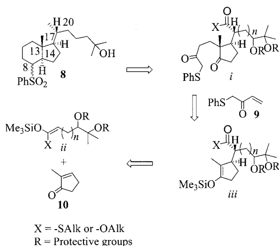
Scheme 2. General plan for the synthesis of 8 from ketene acetals ii and Michael acceptors 10 and 9
