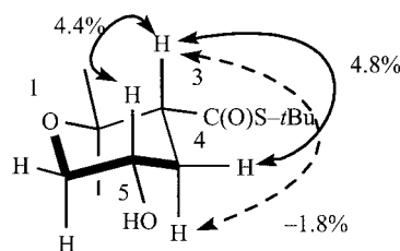
Figure 4. Diagnostic values from a nuclear Overhauser effect (NOE) experiment for 60
