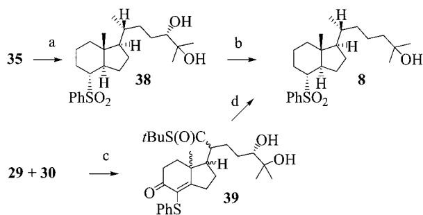
Scheme 8. Transformation of 35 into 8 ; correlation of the structures of diastereomers 29 and 30 . Reagents and conditions, (a) Amberlyst-15H/MeOH, 81%; (b) 1. MsCl/Et 3 N, 2. LiAlH 4 , 87%; (c) 1. KOH/MeOH, 2. HCl, 70%; (d) 1. DIBALH, 2. MsCl/Et 3 N, 3. mCPBA, 4. LiAlH 4 , 26% in 4 steps
