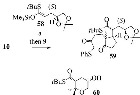
Scheme 11. Attempted synthesis of 8 using ketene acetal 58 . Reagents: (a) \text{TrSbCl}_6 , 39%.
