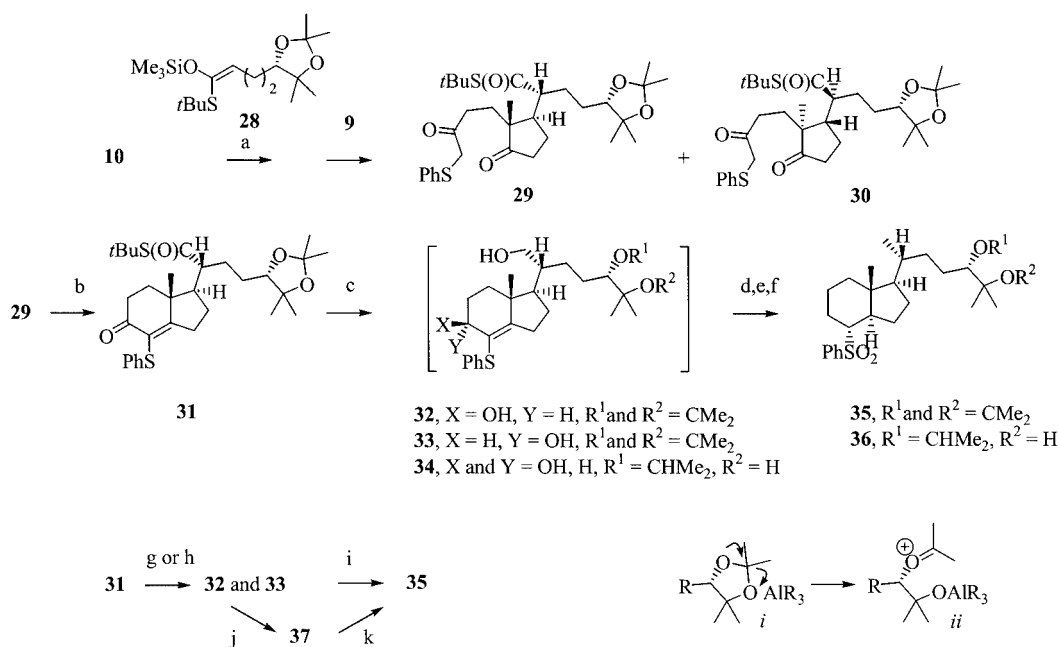
Scheme 7. Synthesis of the CD-rings /side-chain building-block 35 . Reagents and conditions: (a) TrSbCl 6 , cat., 55% yield, then crystallization of 29 ; (b) KOH/MeOH, 84%; (c) DIBALH/CH 2 Cl 2 , -78 °C; (d) TsCl/Et 3 N; (e) m CPBA; (f) LiAlH 4 , 35 , 36% and 36 , 16% from 31 ; (g) 1. CsCl 3 ·H 2 O/NaBH 4 , 2. LiAlH 4 , 32 , 87% and 33 , 5%; (h) as (f), 32 , 73% and 33 , 15%; (i) 1. TsCl, Et 3 N, 2. m CPBA, 3. LiAlH 4 , 70% from 31 ; (j) as (d), 89%; (k) m CPBA and then LiAlH 4 , 72%
