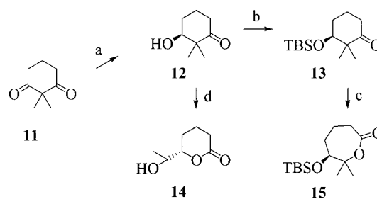
Scheme 3. Synthesis of optically active building-blocks by microbiological reduction of 2,2-dimethylcyclohexan-1,3-dione ( 11 ). Reagents and conditions: (a) Baker's yeast; (b) TBSCl/imidazol/DMF; (c) mCPBA/NaHCO 3 /CH 2 Cl 2 , 87% yield in two steps; (d) mCPBA/CH 2 Cl 2 , 82%
