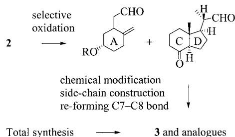
Scheme 1. Convergent synthetic approaches to 1 \alpha ,25-dihydroxyvitamin D 3 and its derivatives
